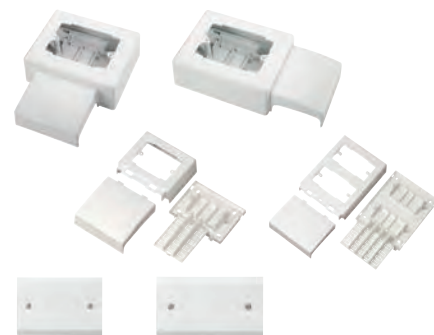
Fittings for trunking 70x20 and 130x28 Series 20 SIMPLY System - MAXI System page 22
